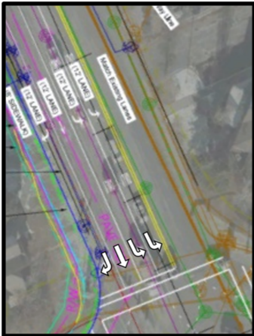
Figure 3: Box of Rock Intersection with two Southbound Left Only Lanes
