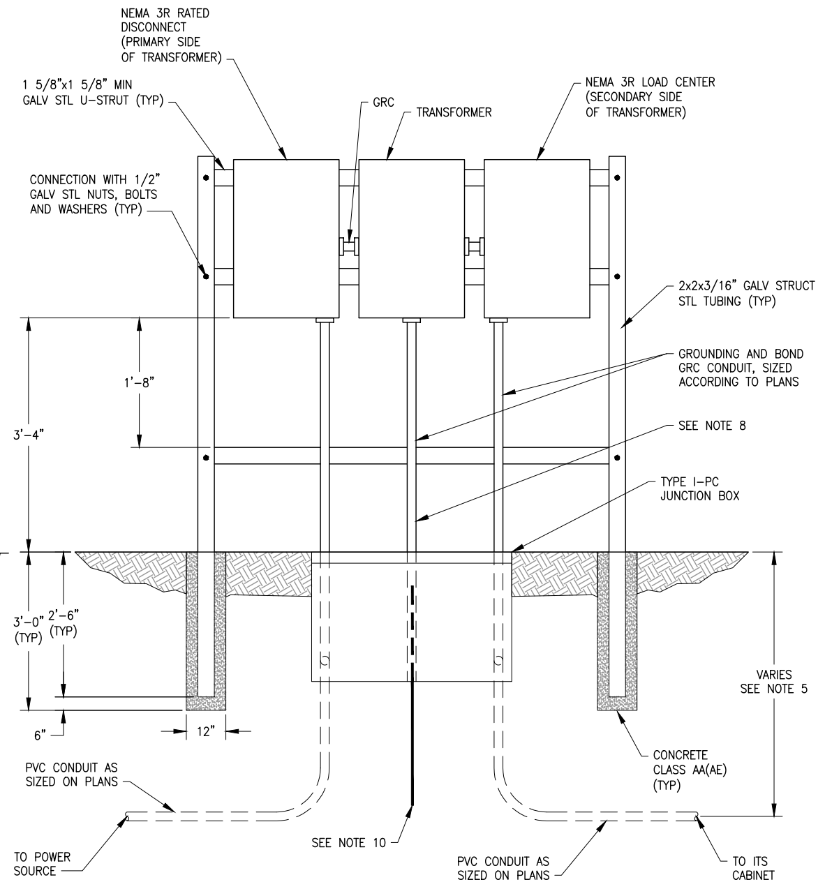
SUPPLEMENTAL DISCONNECT WITH TRANSFORMER FRAME SCALE: NONE (B)
