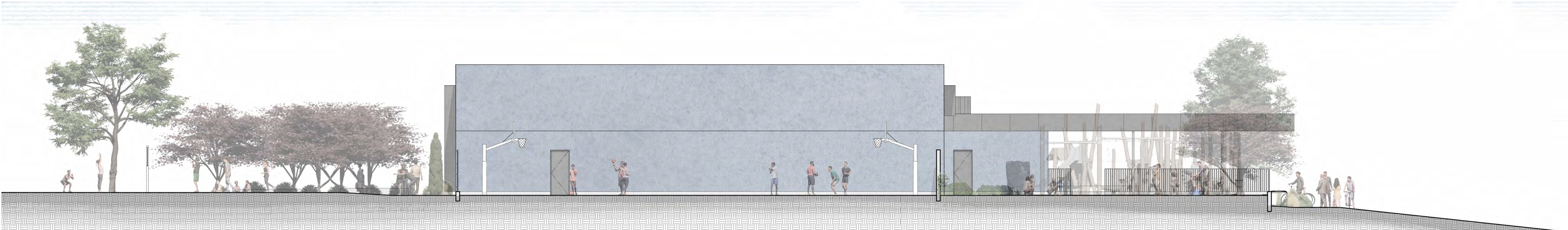
EAST ELEVATION
