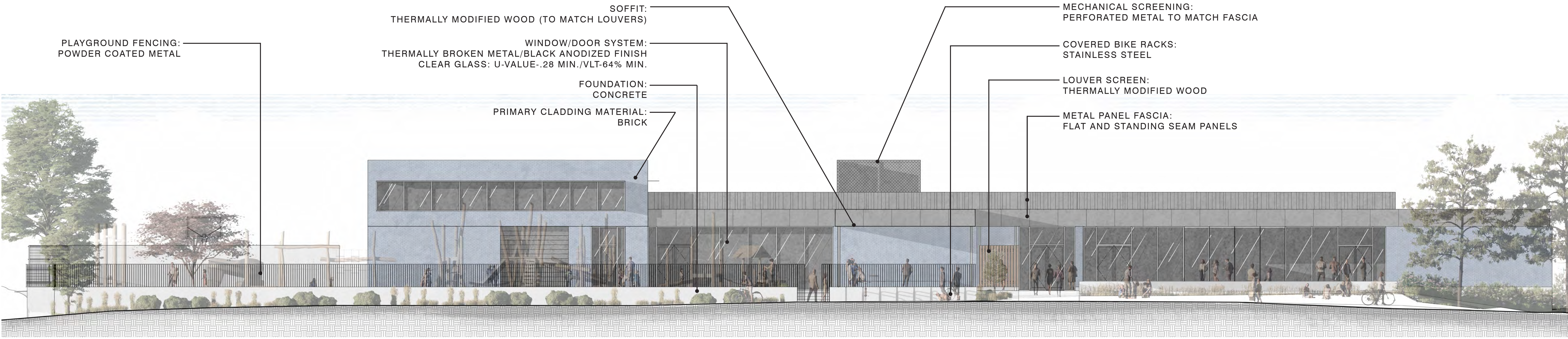
NORTH ELEVATION
