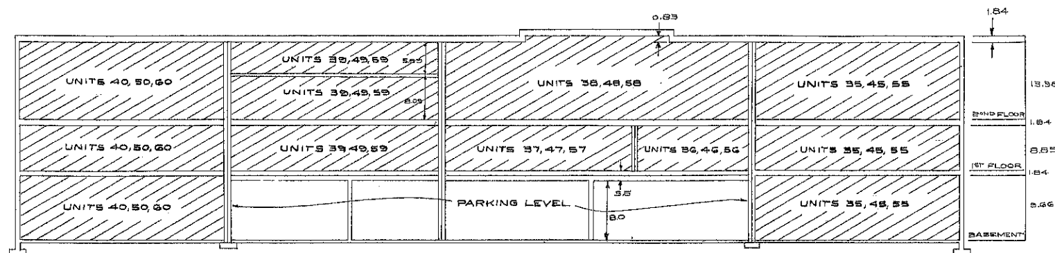
SECTION B
