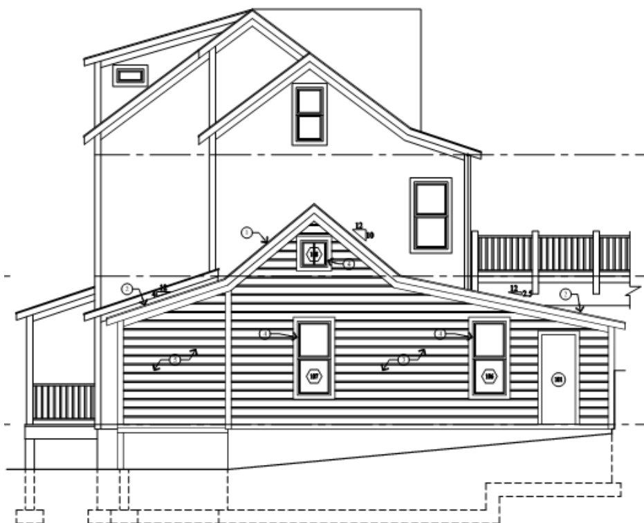
Figure 1d: Current Site Orientation – As-Built Rendering North Façade
